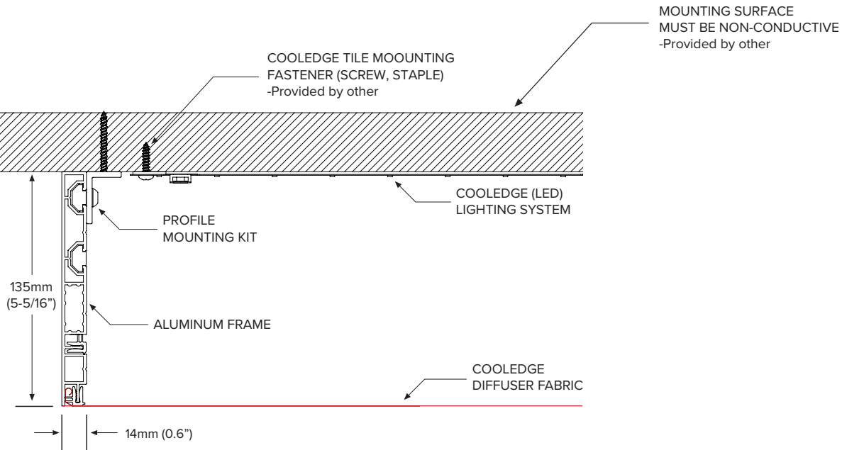
X-Section
