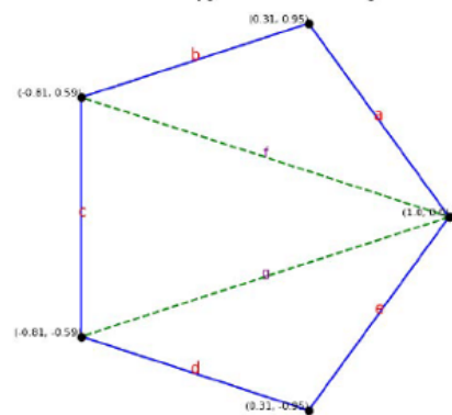
5-sided Polygon with Minimal Diagonals
